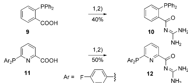
Scheme 4. Synthesis of ligands 10 and 12 : 1) Boc-guanidine (Boc = tert -butoxycarbonyl), N -methylmorpholine, 1-benzotriazolyl-oxyltris(dimethylamino)phosphonium hexafluorophosphate, DMF, RT; 2) trifluoroacetic acid, RT, then Na_2CO_3 , H_2O , CH_2Cl_2 .
