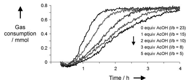
Figure 5. Hydroformylation of 2 ; [Rh(acac)(CO) 2 ]/ 1 / 2 /AcOH = 1:10:200: (0–1000), c 0 ( 2 ) = 0.2 M, THF (2 mL), 10 bar CO/H 2 (1:1), 40 °C, 4 h. Gas consumption curves for increasing amounts of inhibitor AcOH (0–5 equiv relative to substrate 2 ). Regioselectivity (l/b ratio) was determined by 1 H NMR spectroscopic analysis of the reaction mixture.
