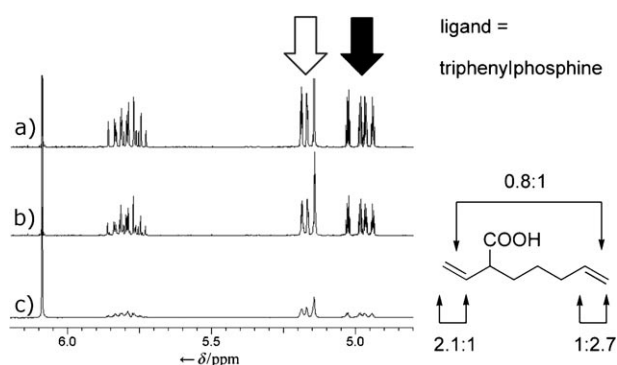
Figure 2. Hydroformylation of 26 using \text{PPh}_3 as a ligand. ^1\text{H} NMR spectra (400 MHz, \text{CDCl}_3 ) of the double-bond region: a) 0 h; b) 9.5 h; c) 25.3 h. Signals from H-2' and H-7 are marked with empty and filled arrows, respectively. Reaction-site selectivity and regioselectivity were determined by ^1\text{H} NMR spectroscopic analysis of the reaction mixture.
