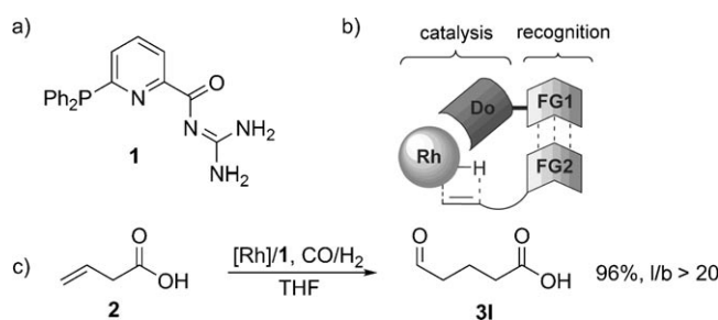
Scheme 1. a) Structure of ligand 1 . [2a] b) Concept of a supramolecular hydroformylation catalyst (Do = donor; FG1,2 = complementary functional groups). c) Regioselective hydroformylation of but-3-enoic acid ( 2 ). [2a]
