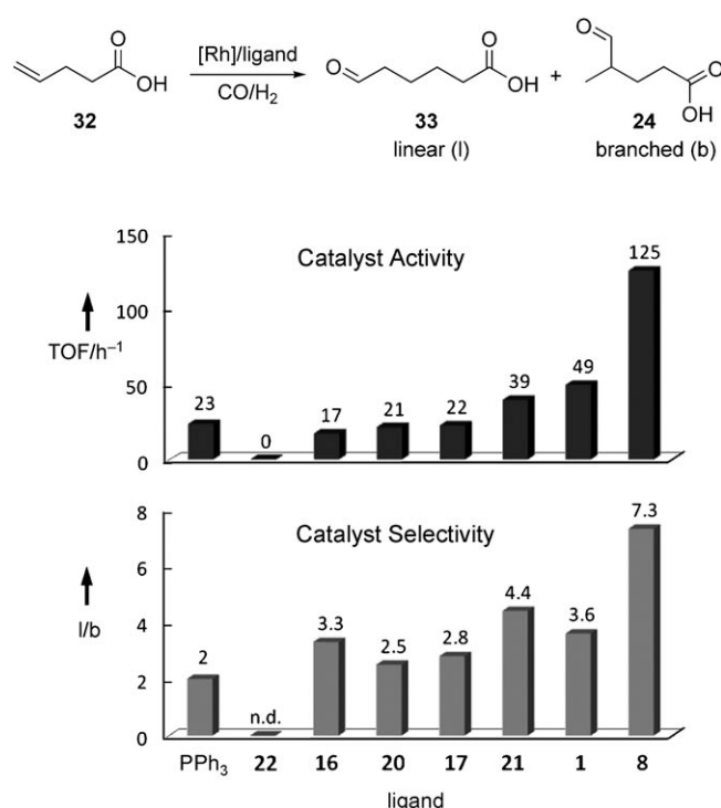
Figure 4. Hydroformylation of 32 . [\text{Rh}(\text{acac})(\text{CO})_2]/\text{ligand}/\mathbf{32} = 1:10:200 , c_0(\mathbf{32}) = 0.2 M, THF (2 mL), 10 bar \text{CO}/\text{H}_2 (1:1), 40 °C, 4 h. TOF (mole aldehyde per mole catalyst per h -1 ) determined from the gas consumption curve. Regioselectivity ( 33 / 24 ratio) was determined by ^1\text{H} NMR spectroscopic analysis of the reaction mixture. n.d. = not determined.
