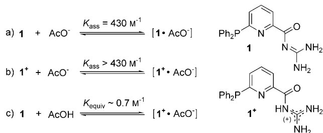
Scheme 10. NMR study of 1 /AcOH interaction ([D 6 ]DMSO, 300 MHz, c_0(\mathbf{1}) = 0.02\text{--}0.03 \text{ M} , RT). [8]
