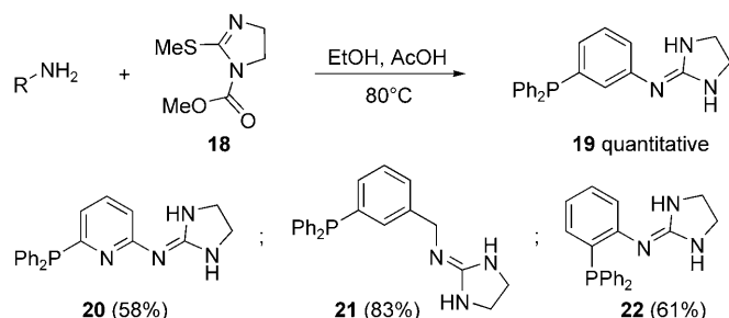
Scheme 6. Synthesis of ligands 19 , 20 , 21 , and 22 .
