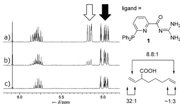
Figure 3. Hydroformylation of 26 using ligand 1 . ^1\text{H} NMR spectra (400 MHz, \text{CDCl}_3 ) of the double-bond region: a) 0 h; b) 4 h; c) 8.5 h. Signals from H2' and H7 are marked with empty and filled arrows, respectively. Reaction-site selectivity and regioselectivity were determined by ^1\text{H} NMR spectroscopic analysis of the reaction mixture.
