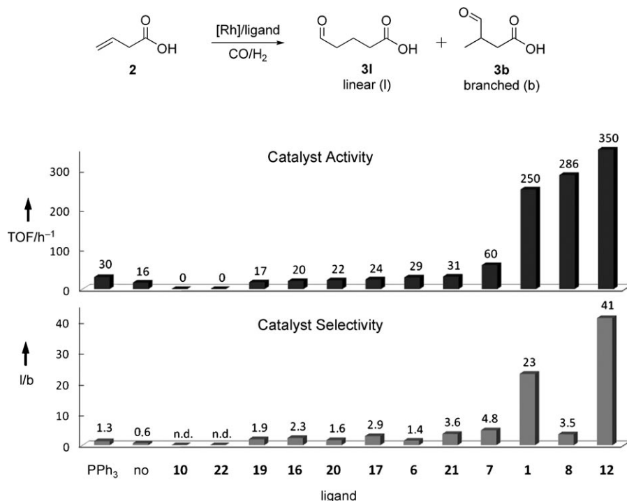
Figure 1. Hydroformylation of 2 ; [\text{Rh}(\text{acac})(\text{CO})_2]/\text{ligand}/\text{2}=1:10:200 (acac=acetylacetonate); c_0(\text{2})=0.2\text{ M} , THF (2 mL), 10 bar \text{CO}/\text{H}_2 (1:1), 40^\circ\text{C} , 4 h. TOF (mole aldehyde per mole catalyst per hour) determined from the gas consumption curve. Regioselectivity, linear/branched ( l/b ) ratio, was determined by ^1\text{H} NMR spectroscopic analysis of the reaction mixture. n.d.=not determined.
