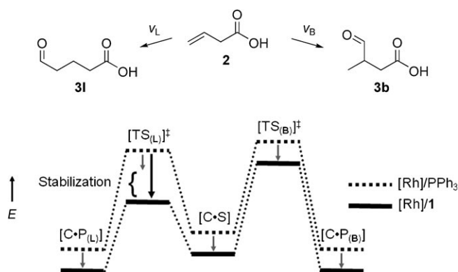
Figure 6. Energy surfaces for the catalyst without (dashed) or with (full) a molecular recognition system. Stabilization imparted by supramolecular interaction marked with arrows, [C·S] or [C·P] represents catalyst–substrate (product) adduct, [TS(L)] ‡ and [TS(B)] ‡ represent the corresponding transition states. Selective lowering of the energy barrier is marked with a black parenthesis.
