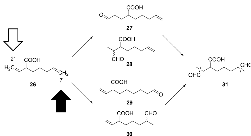
Scheme 7. Hydroformylation of 26 ; [Rh(acac)(CO) 2 ]/ligand/ 26 = 1:10:150; c 0 ( 26 ) = 0.2 M, THF (8 mL), 4 bar CO/H 2 (1:1), 25 °C.
