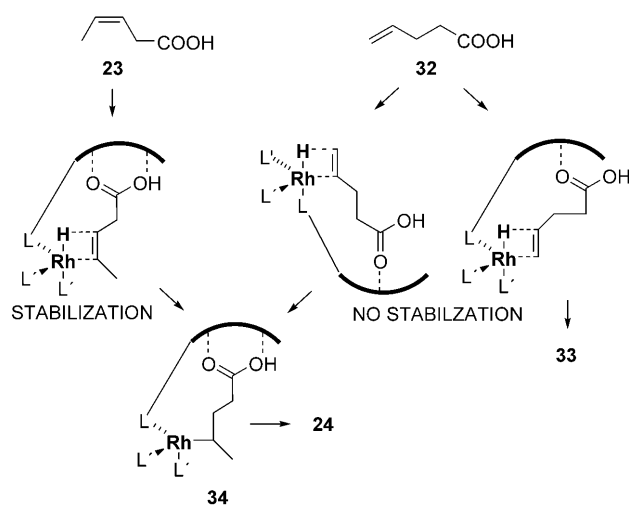
Scheme 8. Substrate binding in the rate- and selectivity-determining hydrometalation step for substrates 23 and 32 . The bold curve represents the substrate binding site of ligand 1 .
