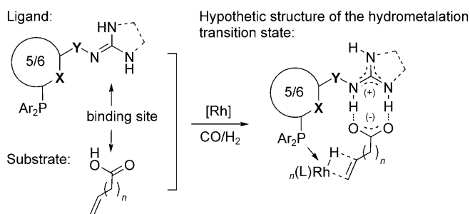
Scheme 2. Design of guanidine ligands for supramolecular catalysis, generalized structure of ligand ( X=N, CH, NH ; Y=CO, CH_2 , or no linker) and substrate. Hypothetical structure of the hydrometalation transition state.
