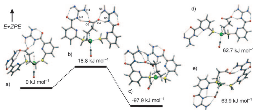
Figure 7. DFT calculations on the reaction mechanism of directed hydroformylation of 2 . a) Catalyst–substrate complex; b) transition state of hydrometalation; c) catalyst–product complex; d, e) alternative transition states. E + ZPE = electronic energy + zero point energy (relative to structure a ).
