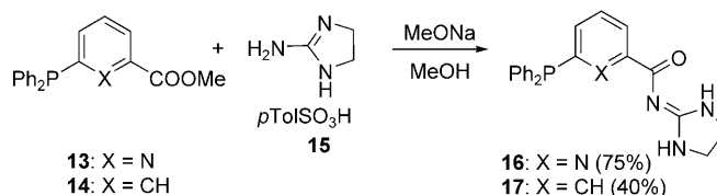
Scheme 5. Synthesis of ligands 16 and 17 .
