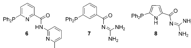
Scheme 3. Previously reported ligands 6 , [2a] 7 , [2a] and 8 . [3]
